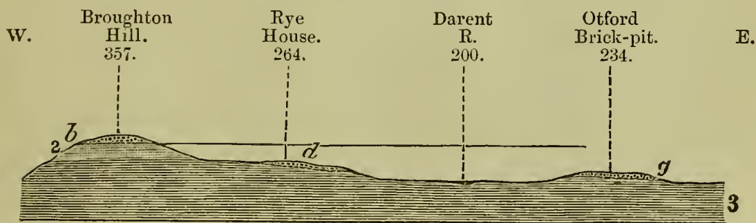
Fig. 10.—Section from Dunton Green to the Otford and Sevenoaks Road.
